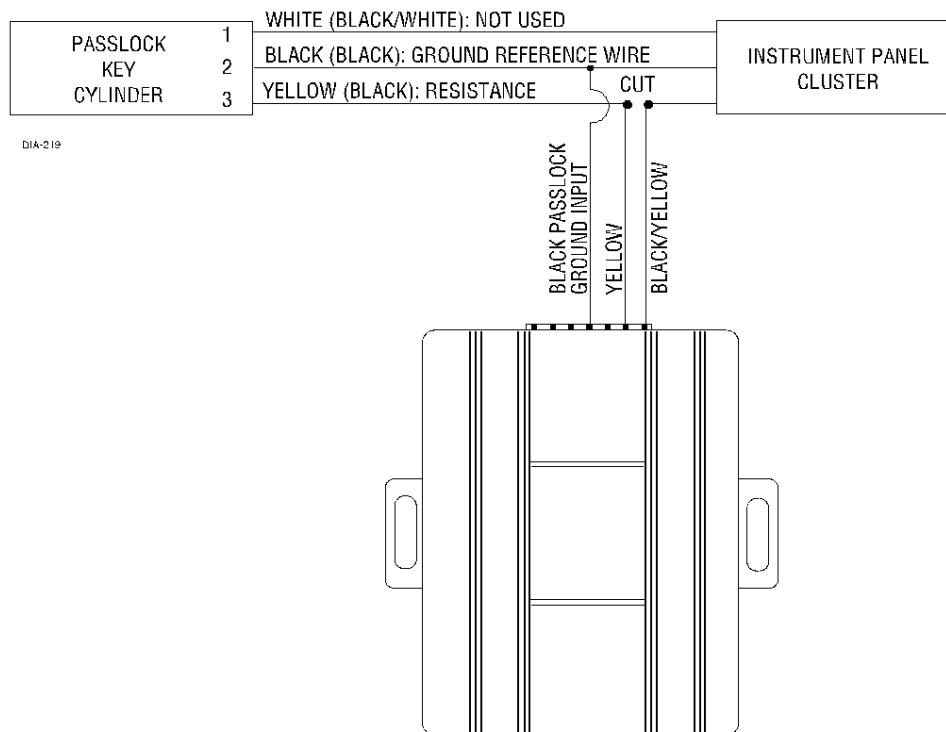
THREE-WIRE PASSLOCK CABLE
